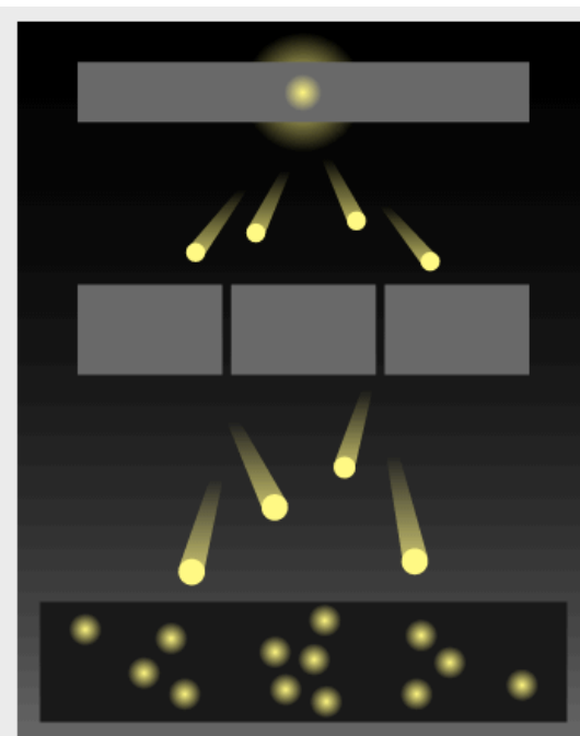
7.6.3 • An interference pattern can be built up over time by a series of single photons passing through Young's experiment, demonstrating the wave-particle duality of light.
