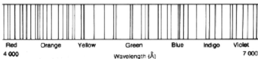
The solar spectrum.
